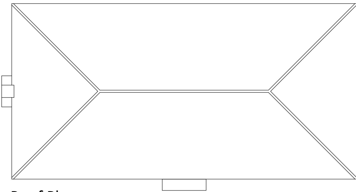
Roof Plan
