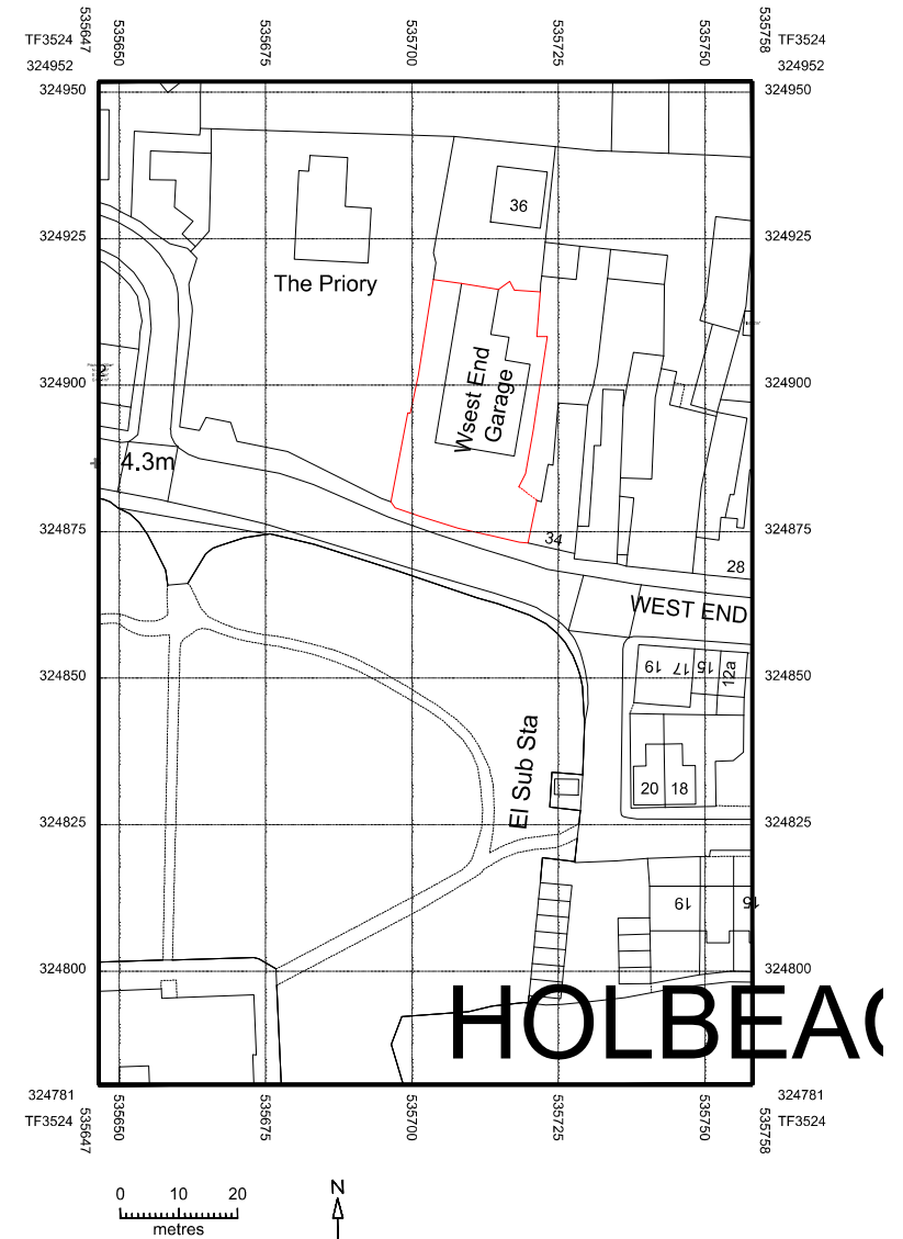
LOCATION PLAN SCALE 1:500
