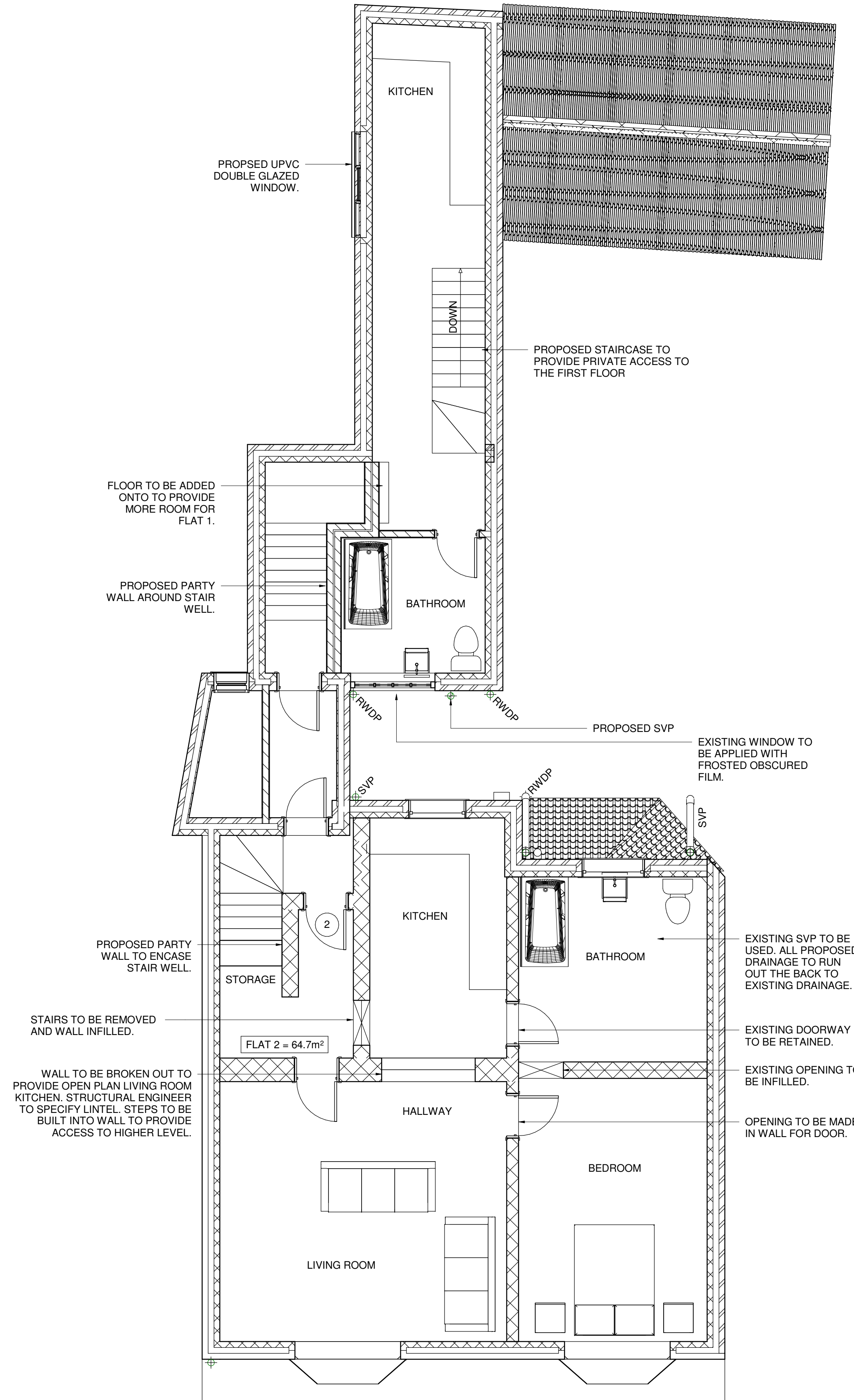
PROPOSED FIRST FLOOR SCALE: 1 : 50
