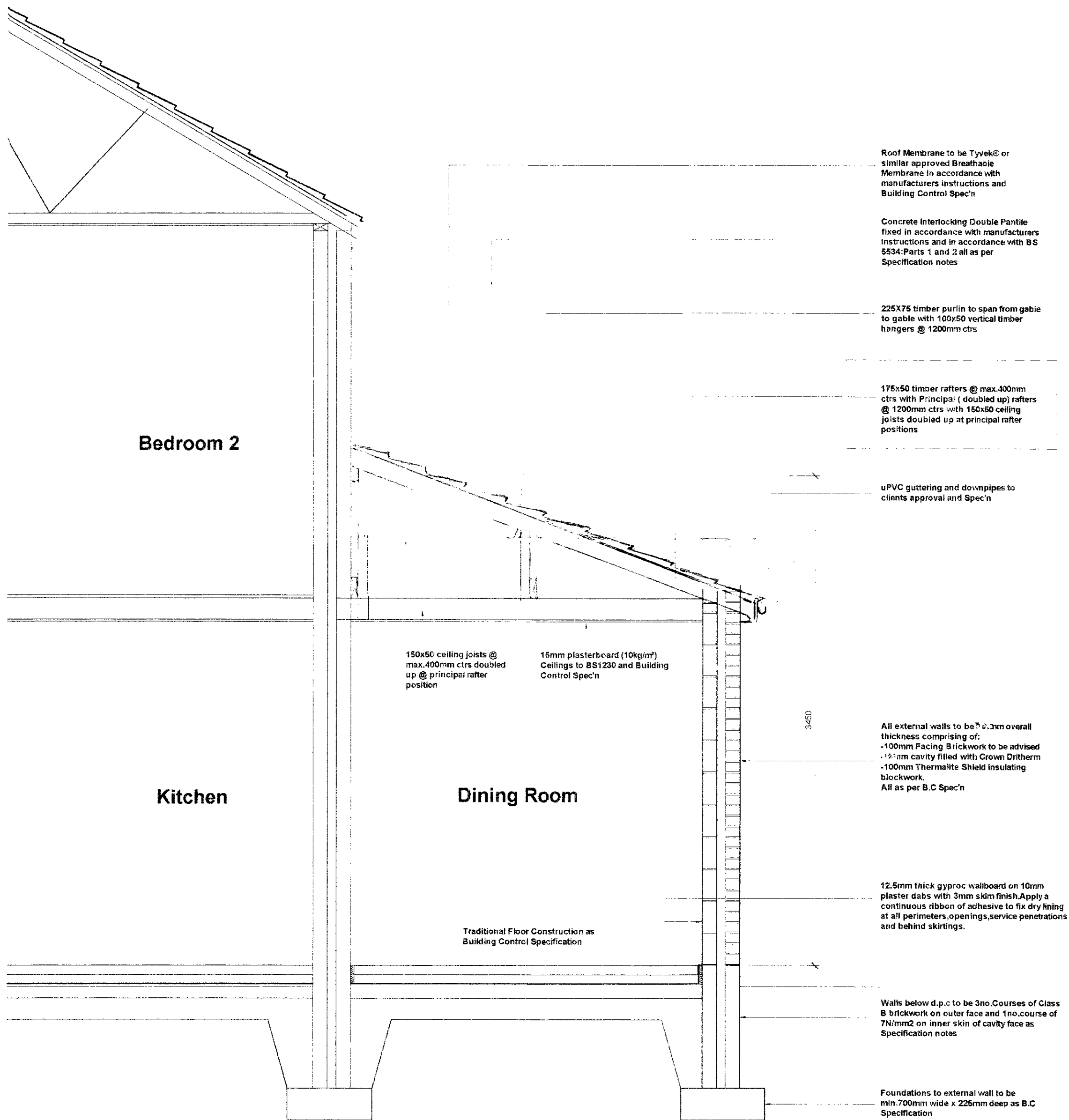
Section B-B Scale 1:25
