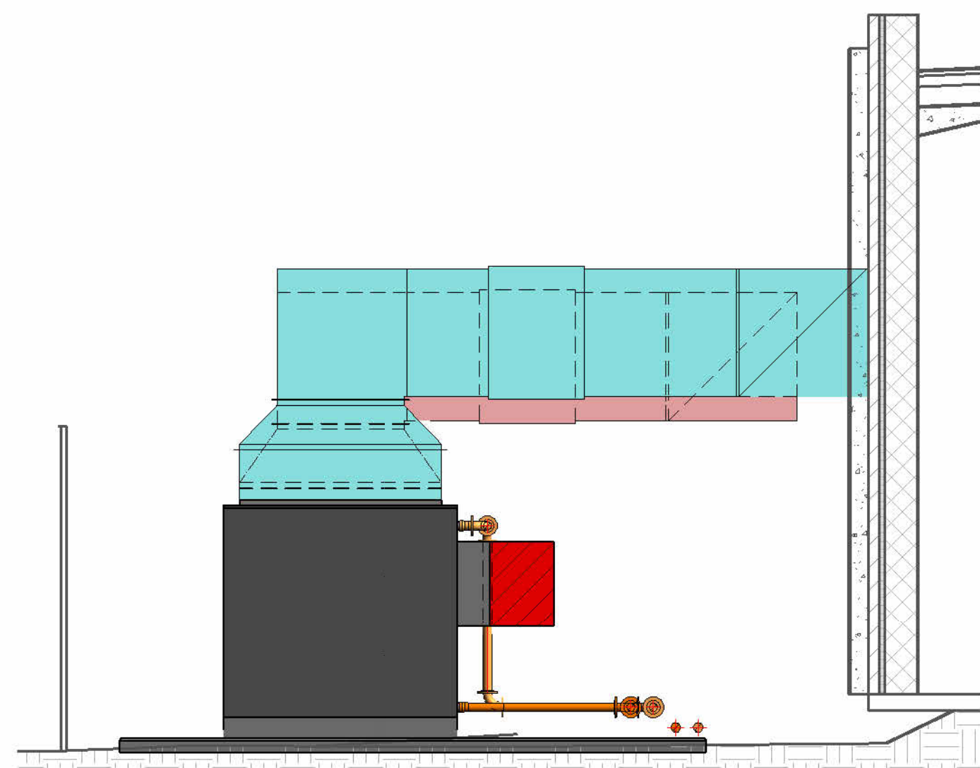
SECTION A - AHU.01 1:50
