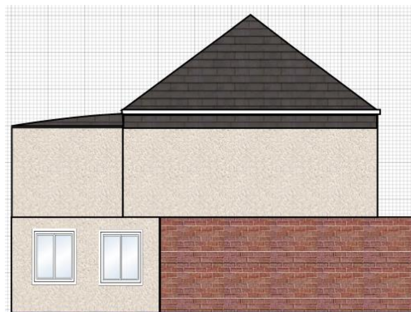
EAST ELEVATION AS PROPOSED
