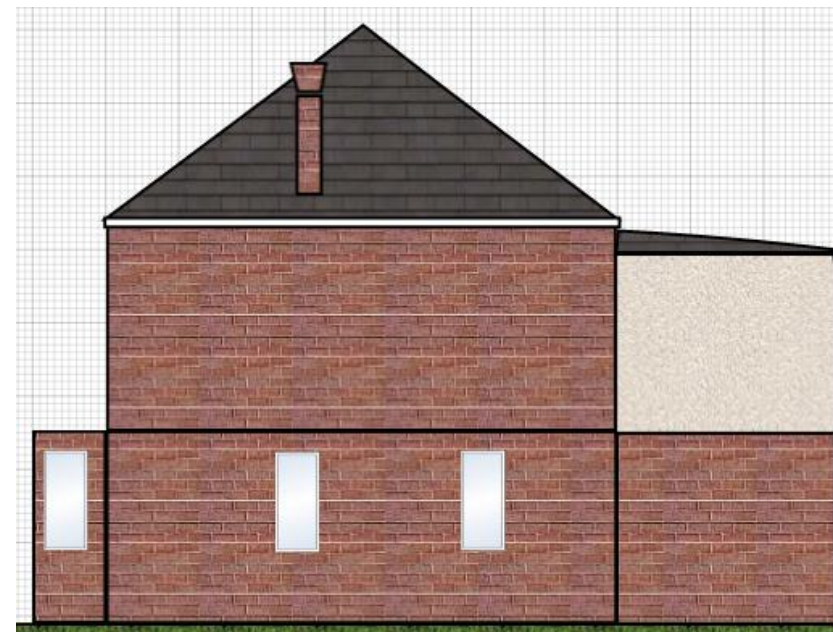
WEST ELEVATION AS PROPOSED
