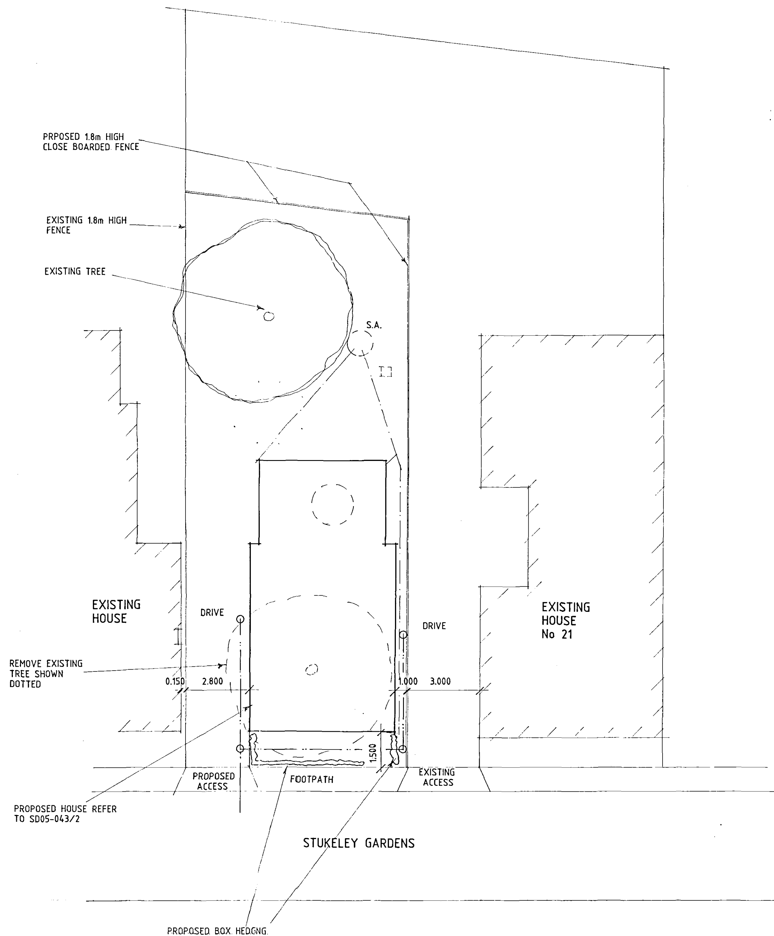
SITE PLAN
