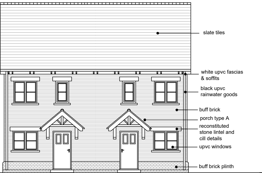
FRONT ELEVATION
