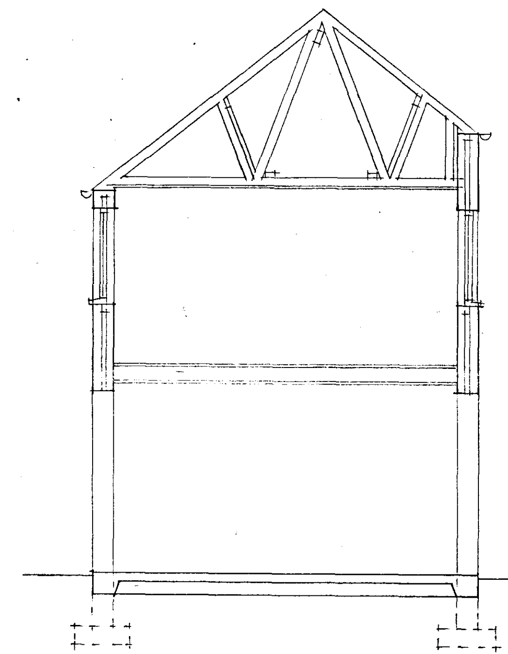
SECTION
