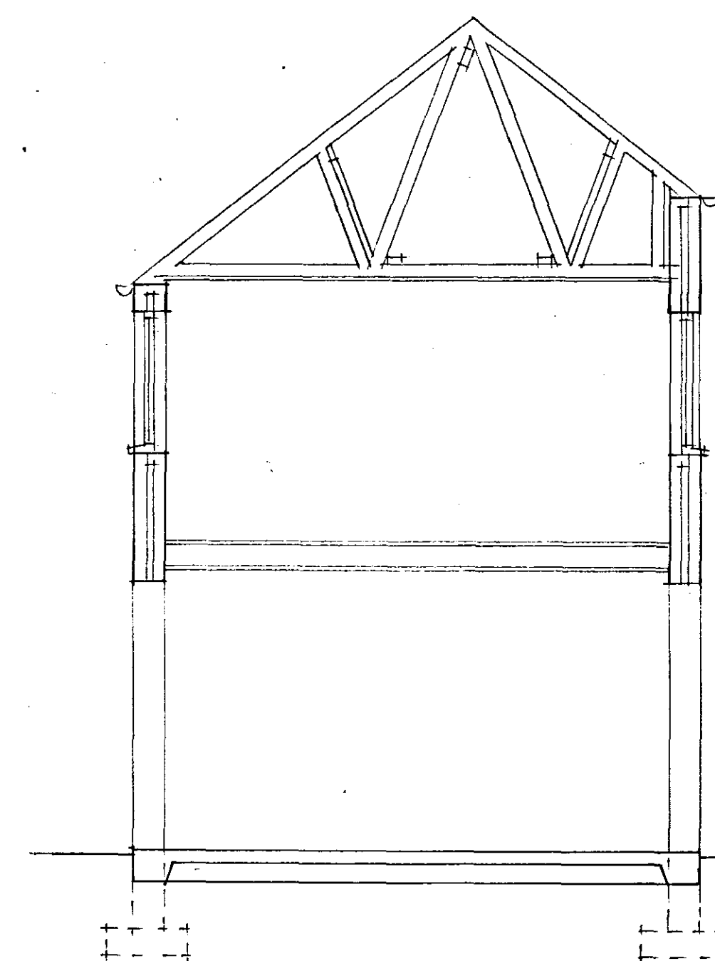
SECTION
