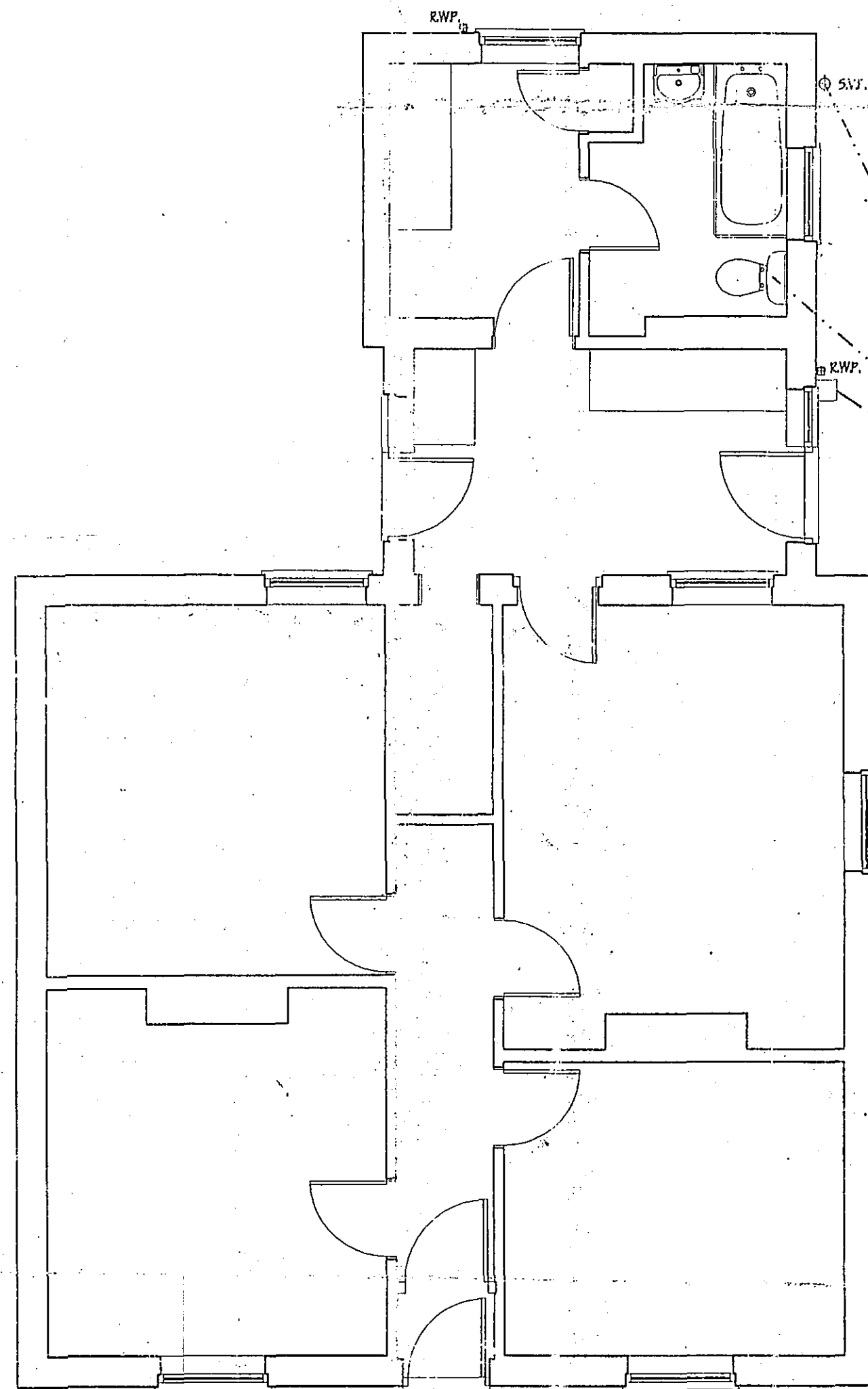
FLOOR PLAN (EXISTING)
