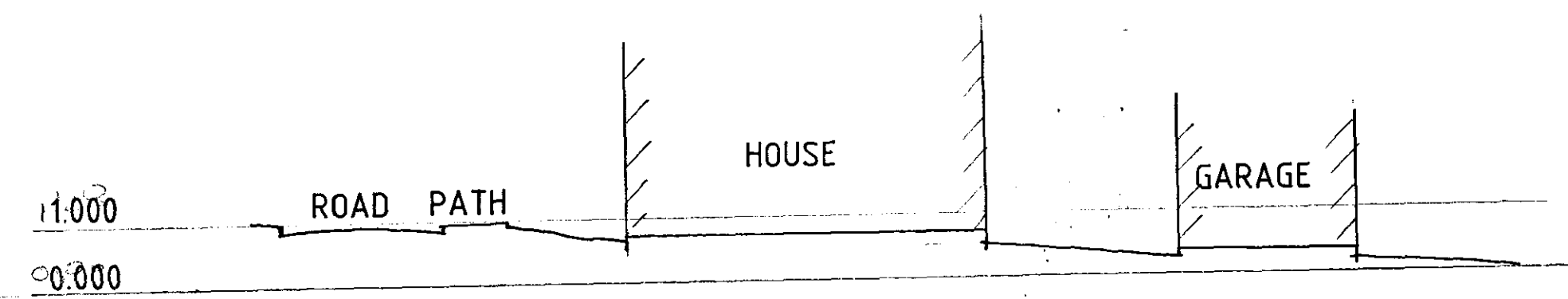
SECTION THRO SITE
