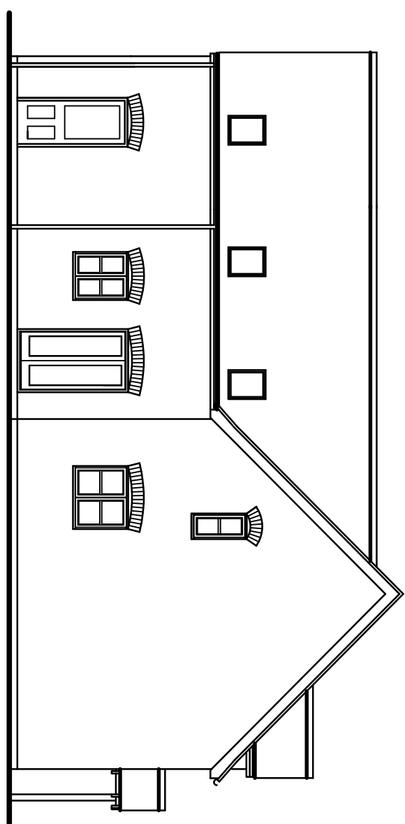
SIDE ELEVATION
