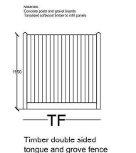
Timber double sided tongue and groove fence
