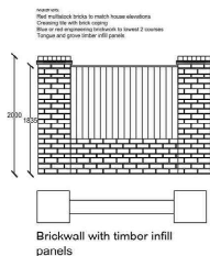
Brick wall with timber infill panels
