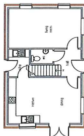
Ground Floor Layout (50m2 / 538sqft GFA)
