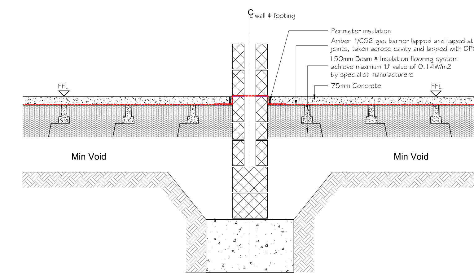
Typical Strip Section B-B scale 1:20
