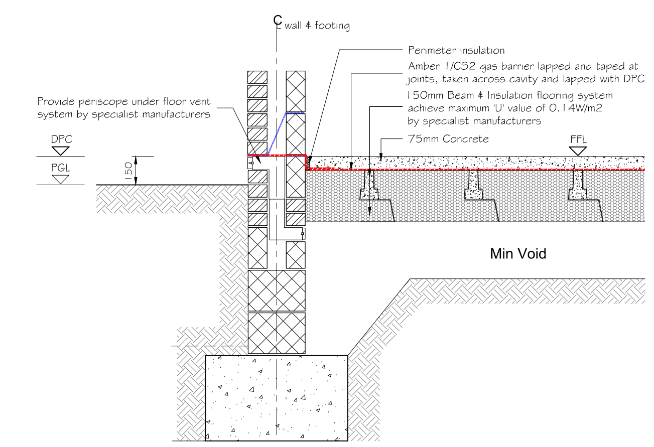
Typical Strip Section A-A scale 1:20
