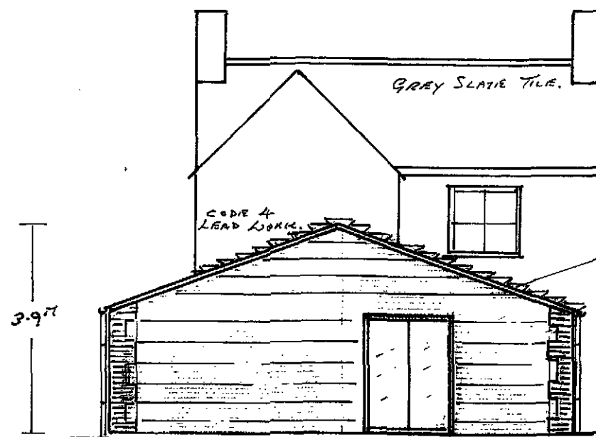
REAR SOUTH
