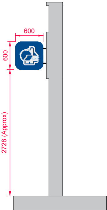
PROPOSED SIDE SECTION
