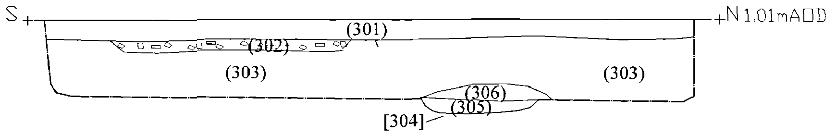
Trench 3 Section
