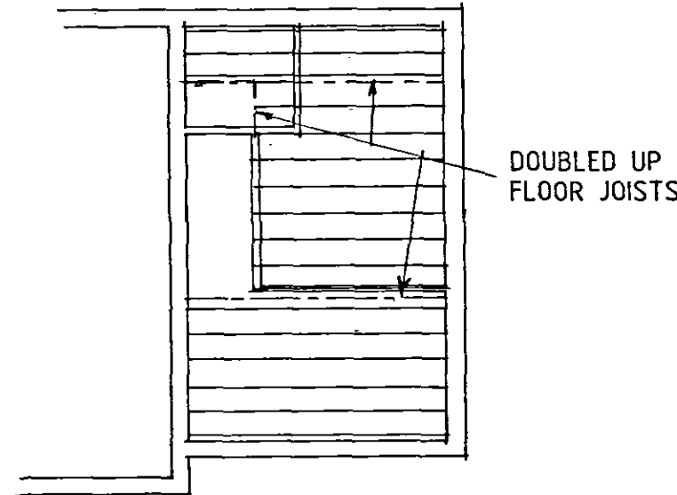
FIRST FLOOR JOIST PLAN
