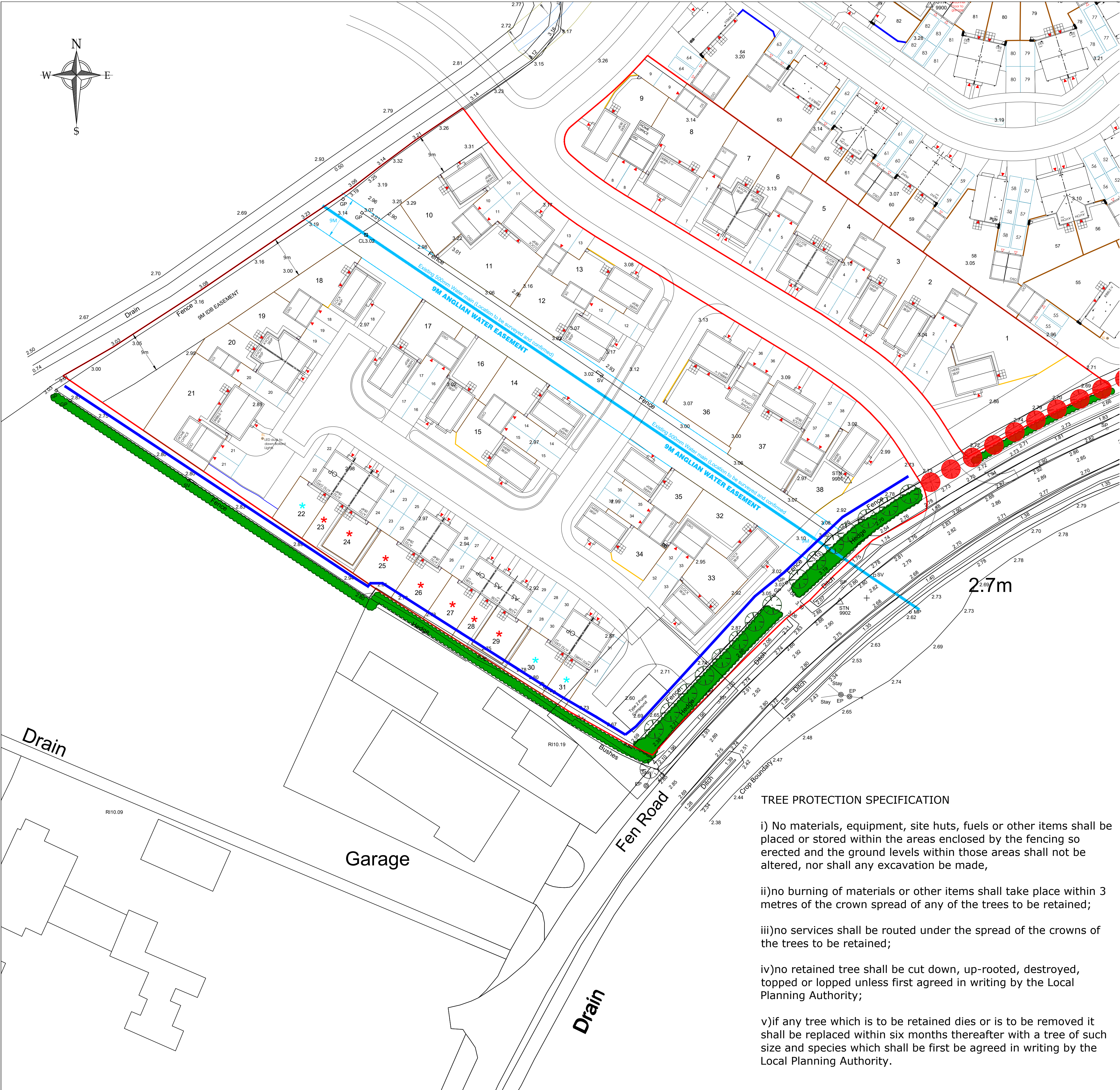
Proposed Tree Protection Fencing
