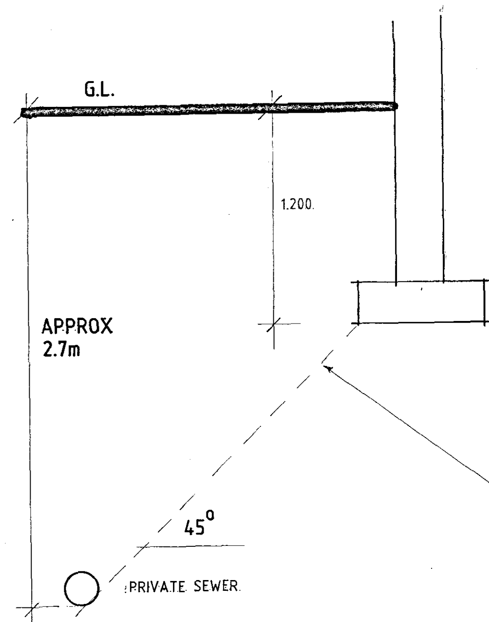
SECTION THRO PRIVATE SEWER & FOUNDATION
