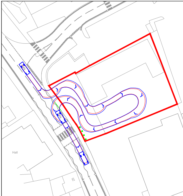
6.4t LIGHT VAN TRACKING (1:1000)
