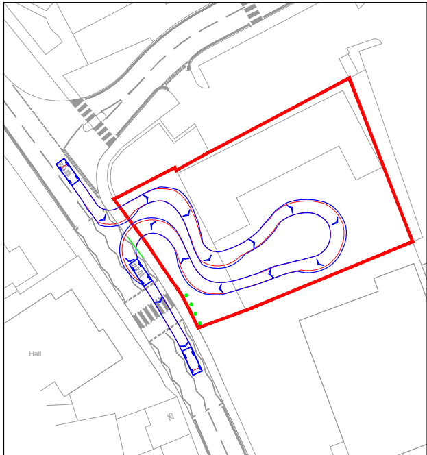
LARGE CAR TRACKING (1:1000)
