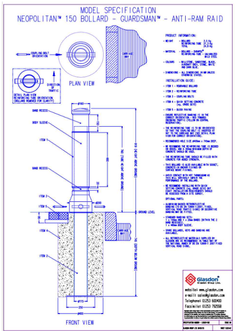
BOLLARD SPECIFICATION
