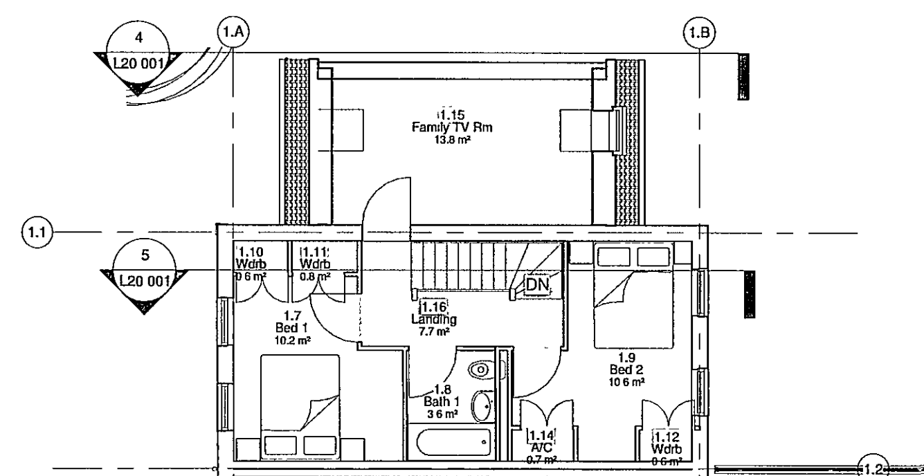
Type 1 6p House Level 2 1 : 100
