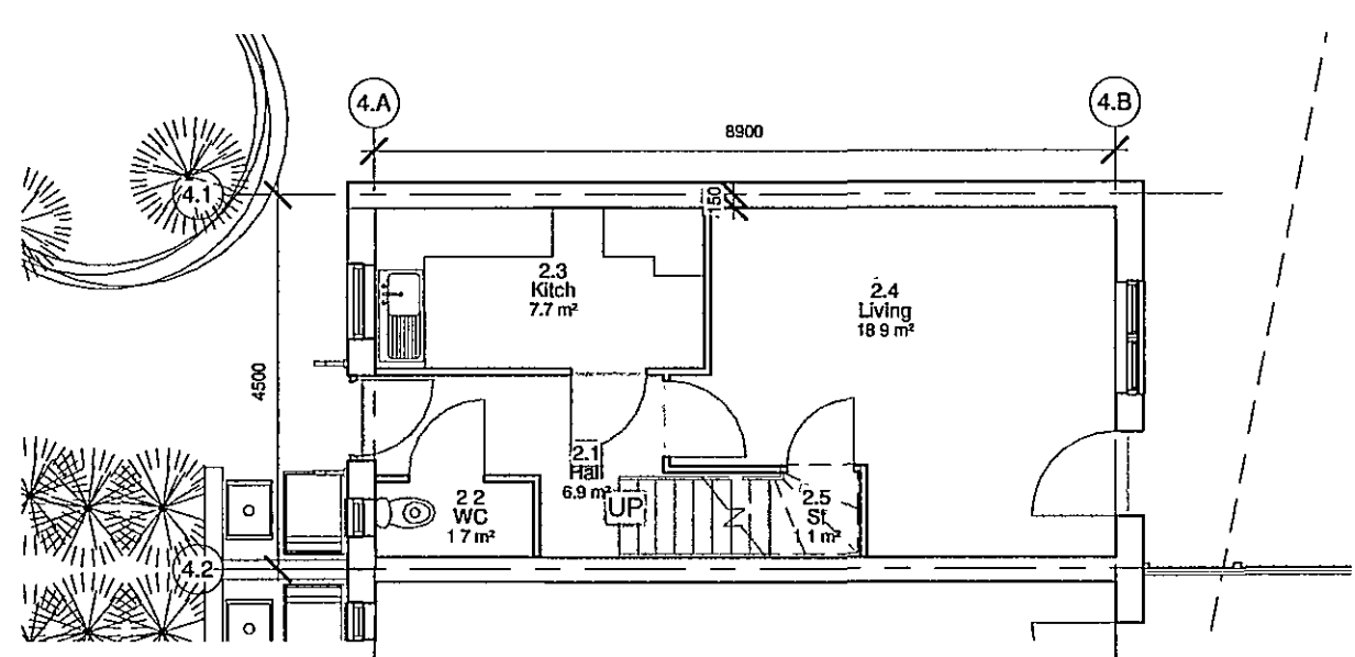
Type 2 4p House Level 1 1 : 100
