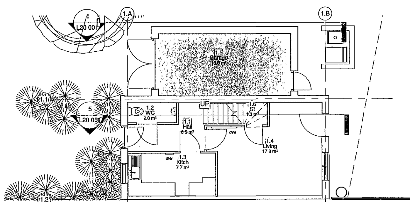
Type 1 6p House Level 1 1 : 100
