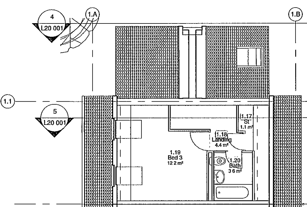
Type 1 6p house Level 3 1 : 100
