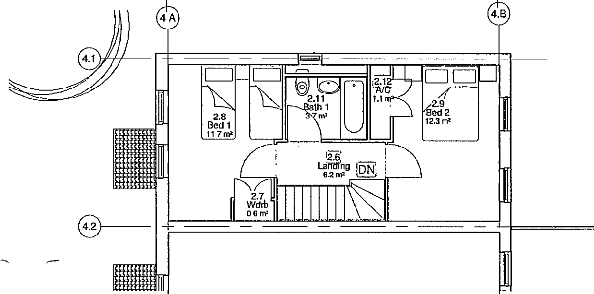
Type 2 4p House Level 2 1 : 100
