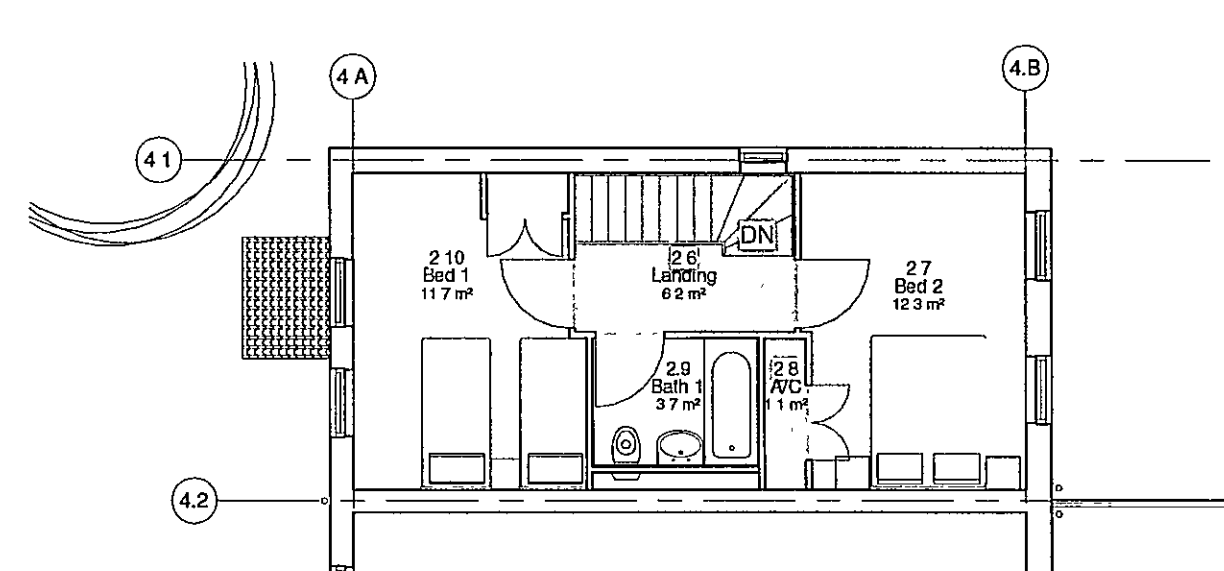
Type 2 4p House Level 2 1 : 100
