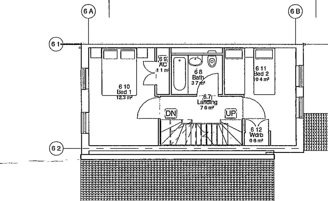
Type 2 4p House Level 2 1 : 100
