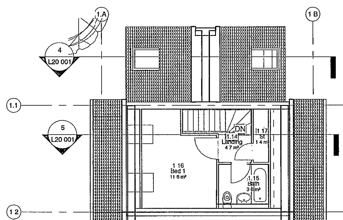
Type 1 6p house Level 3 1 : 100
