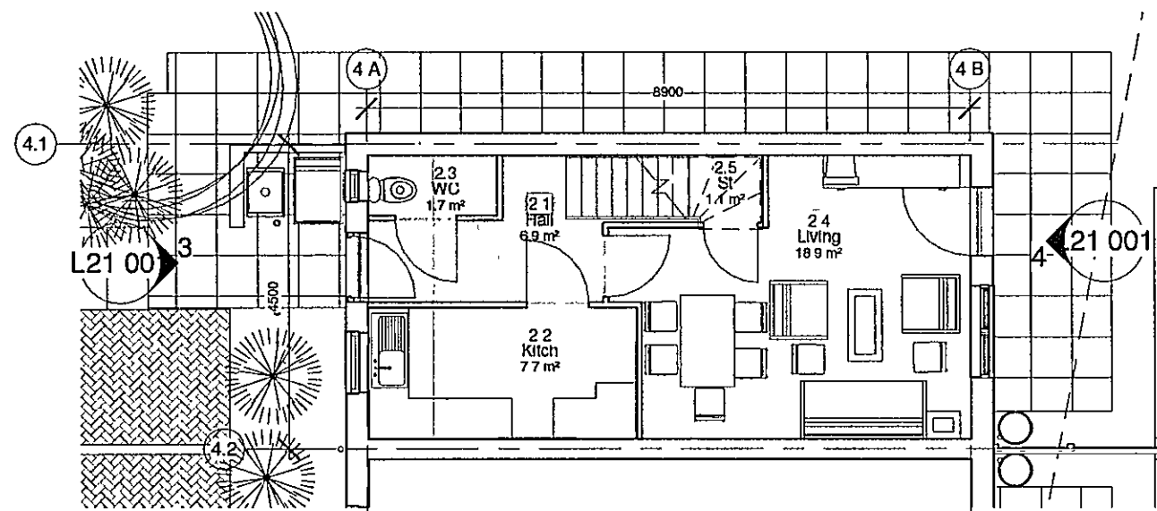
Type 2 4p House Level 1 1 : 100
