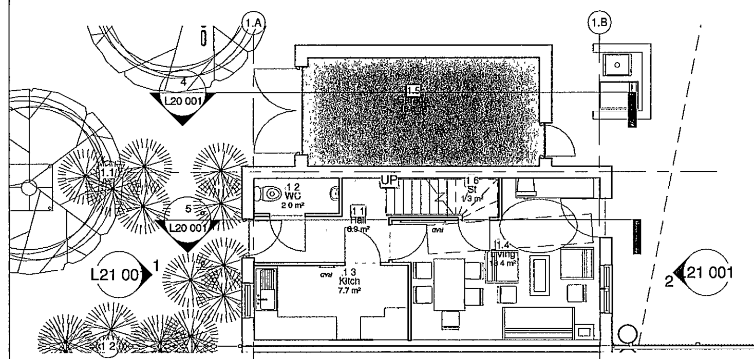
Type 1 6p House Level 1 1 : 100
