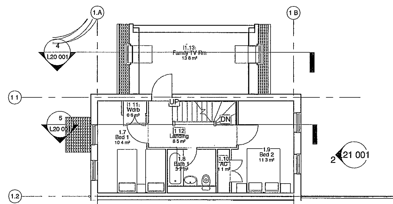
Type 1 6p House Level 2 1 : 100
