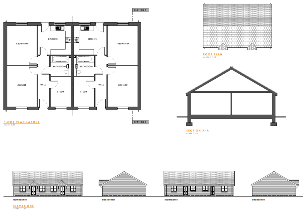
Figure 3 - Proposed dwellings.
