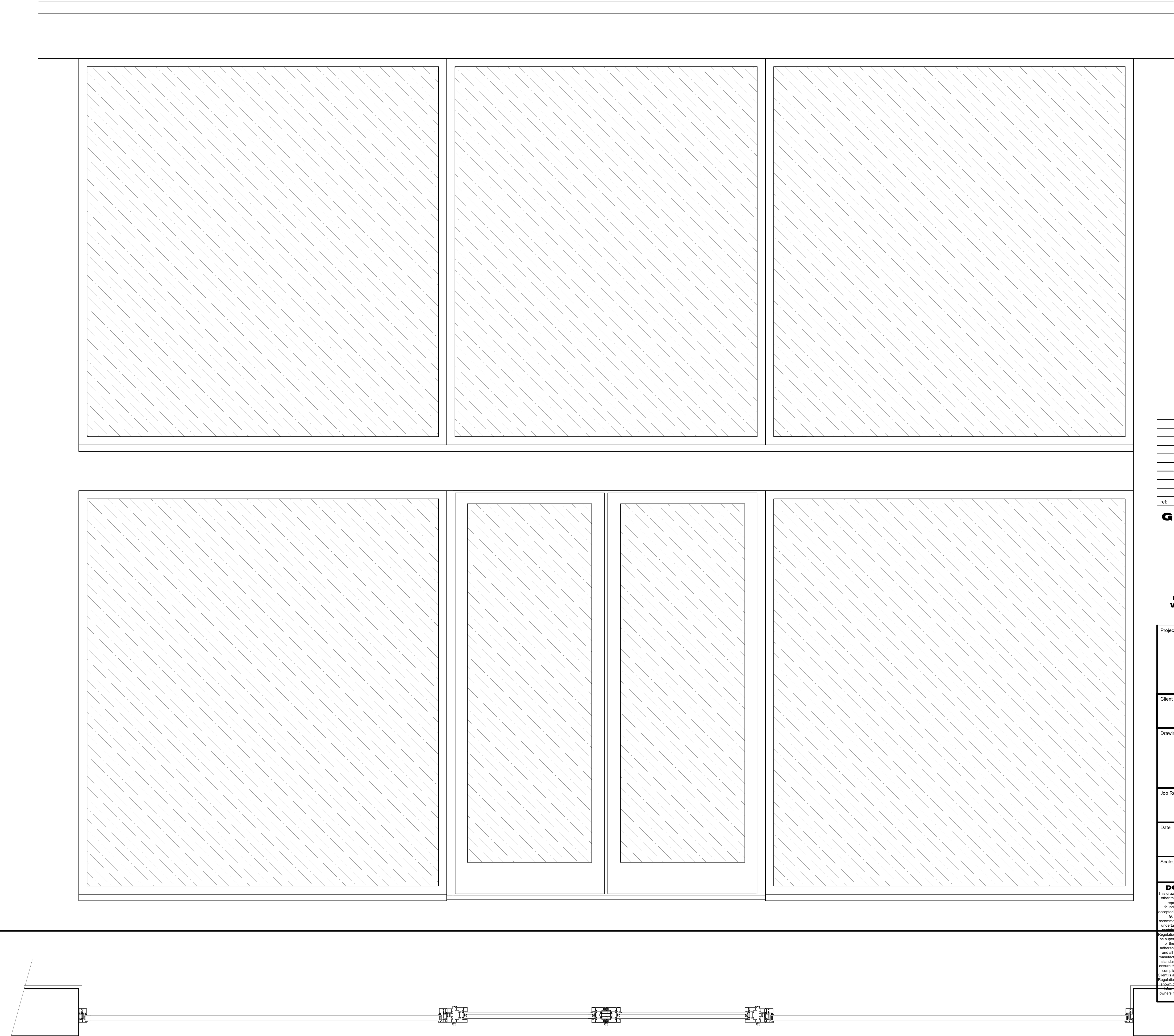
ALUMINIUM DOOR AND GLAZED SCREEN FRAME DETAILS 1:10
