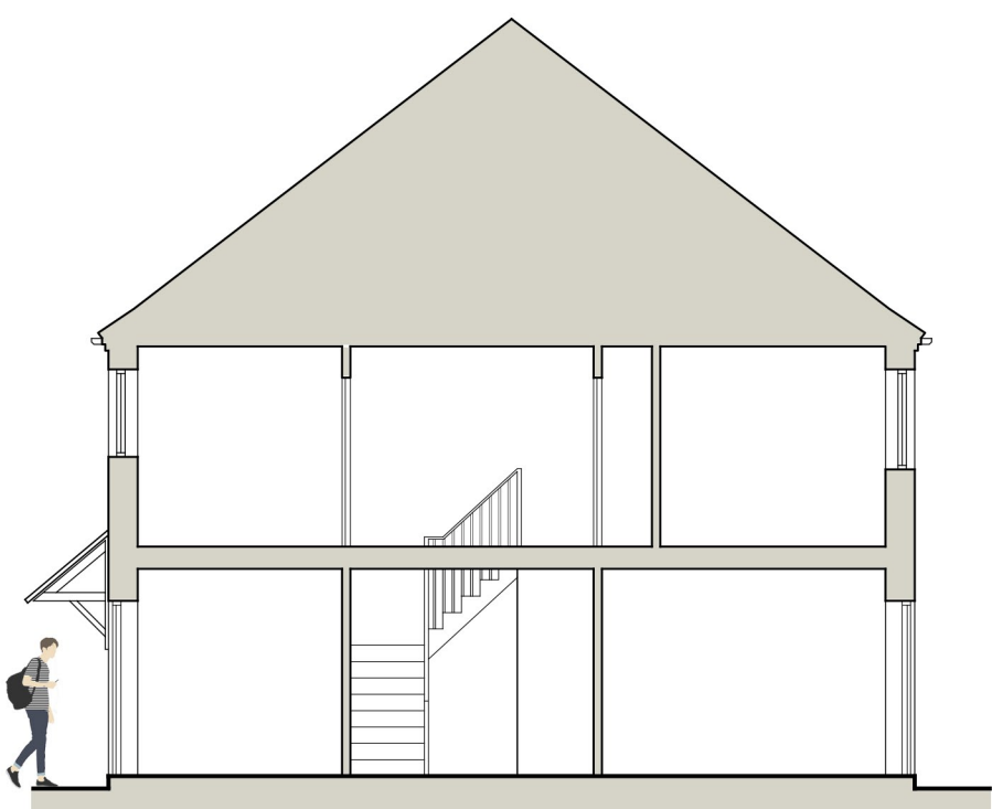
Section B-B
