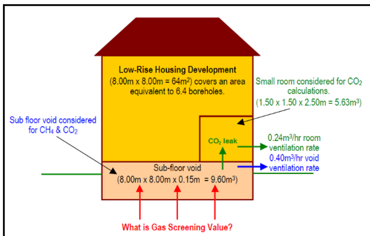
Figure F1: Model Residential Property Developed for Calculating Maximum Permitted Equilibrium Gas Concentrations within the Sub-Floor Void
