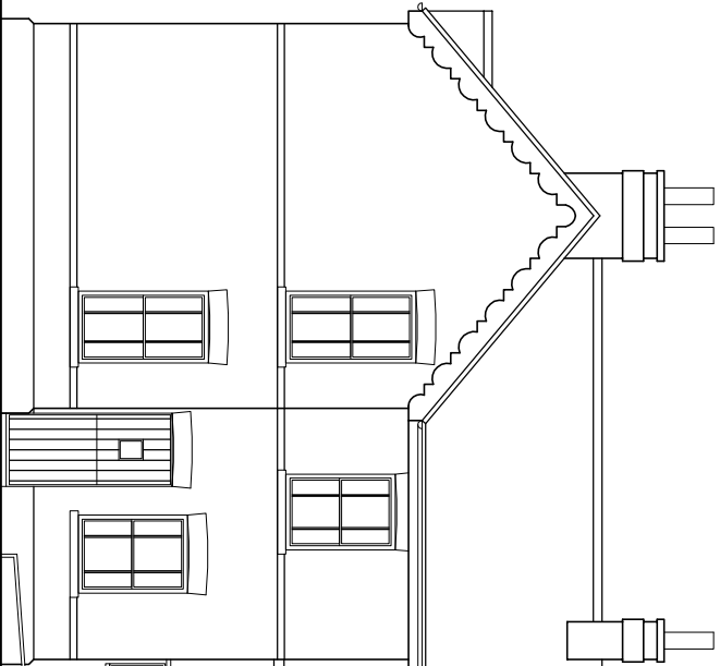
SIDE ELEVATION
