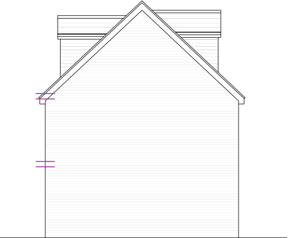
WEST ELEVATION @ 1:100
