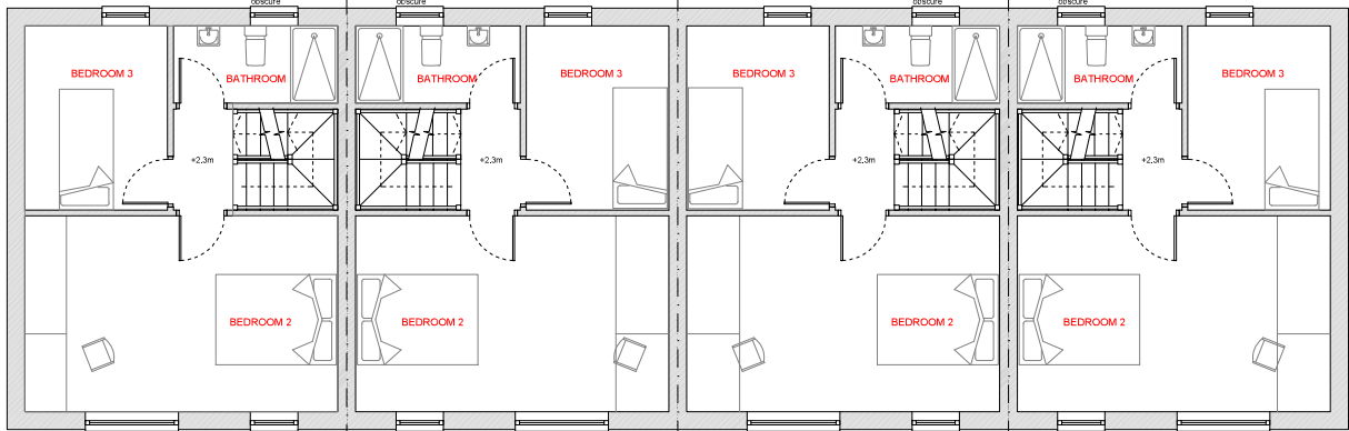
FIRST FLOOR PLAN @ 1:100
