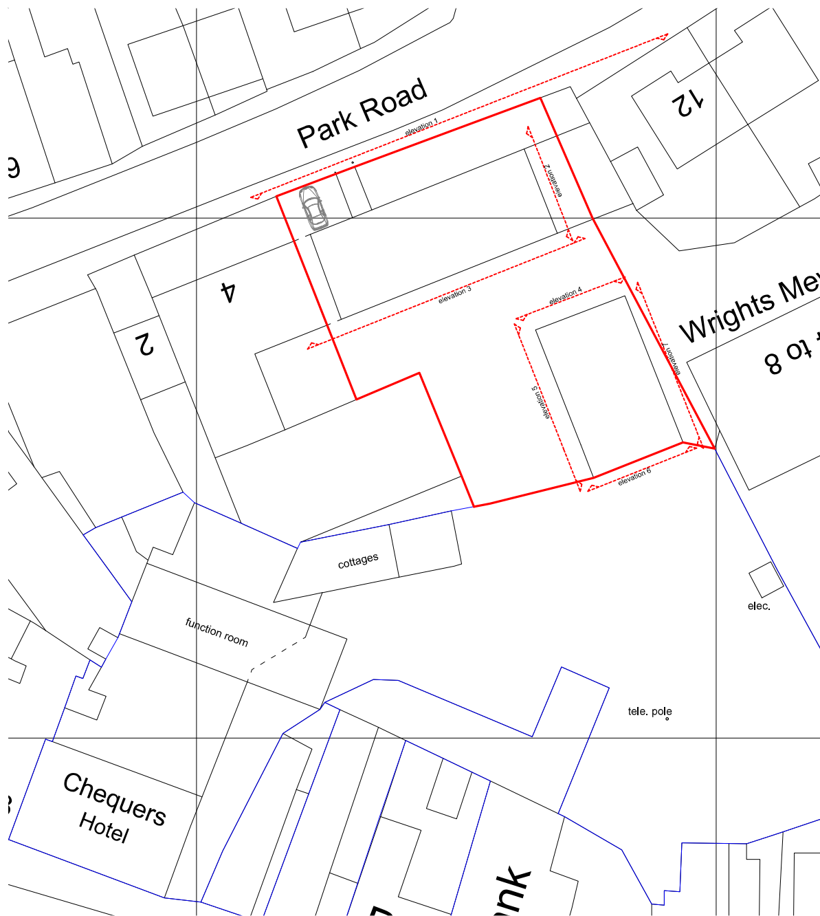
SITE PLAN @ 1:500
