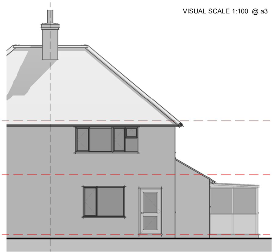
Elevation 01 - Front 1 : 100
