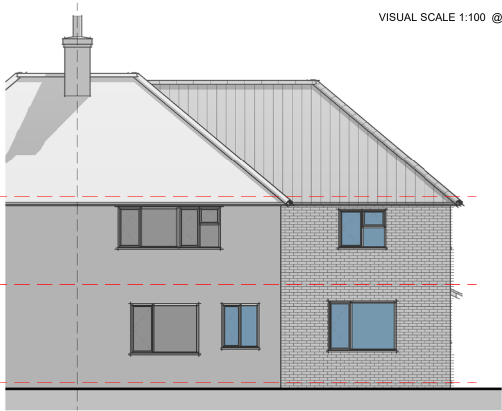
Elevation 01 - Front 1 : 100
