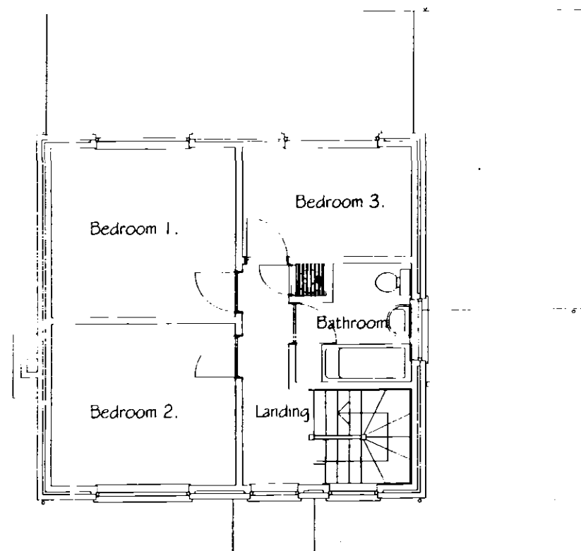
FIRST FLOOR PLAN EXISTING
