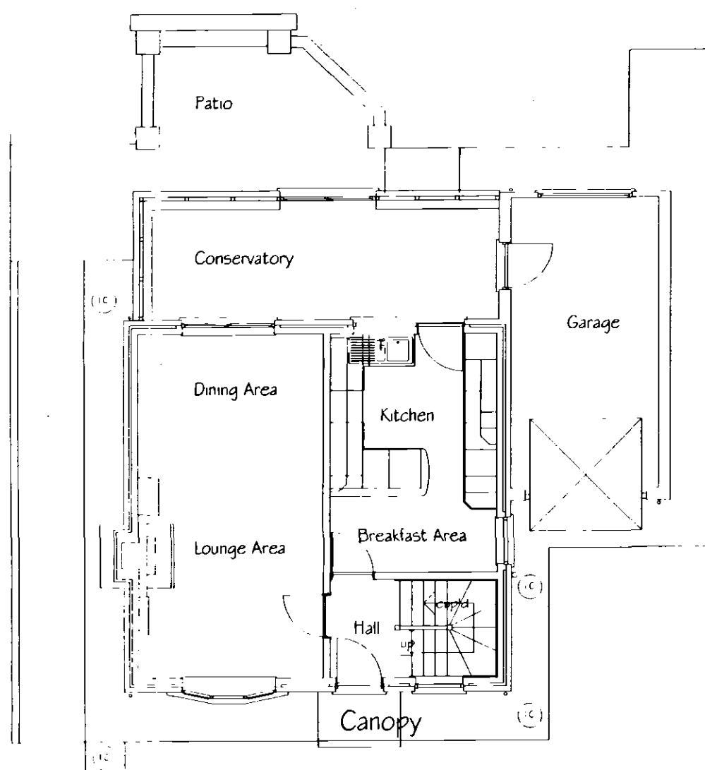
GROUND FLOOR PLAN EXISTING
