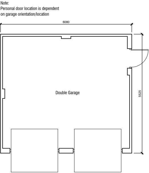
Double Garage Plan
