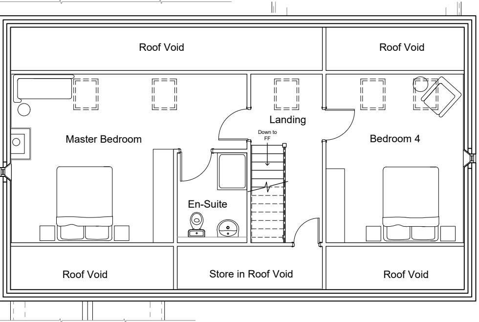
Second Floor/Attic Plan
