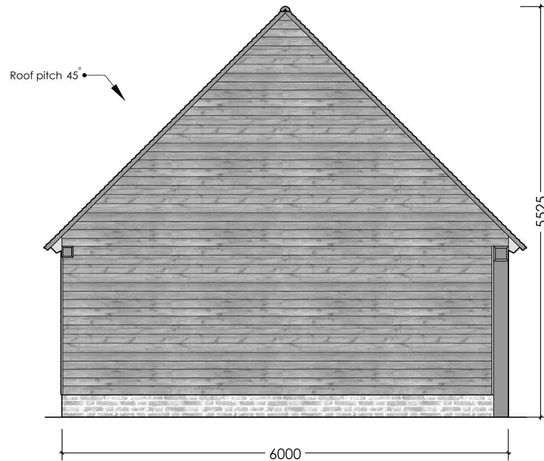
Left Elevation
