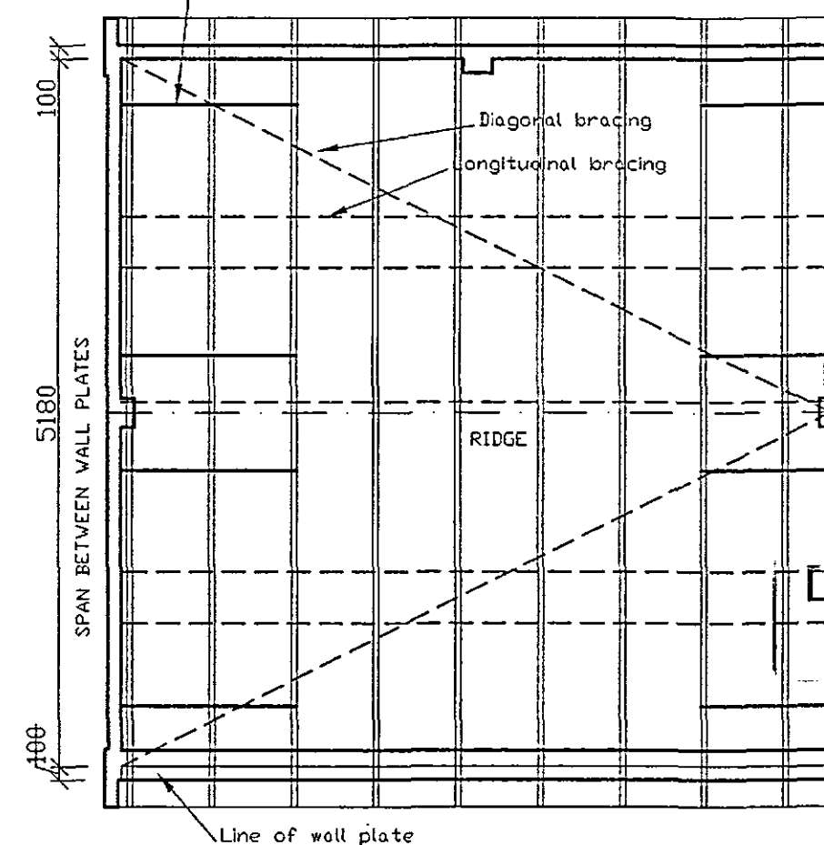
TRUSS LAYOUT
