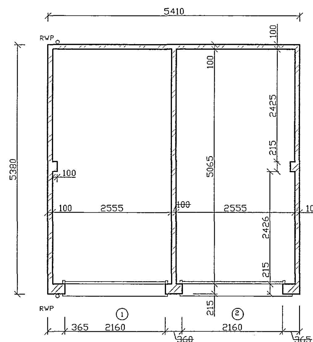
FLOOR PLAN
