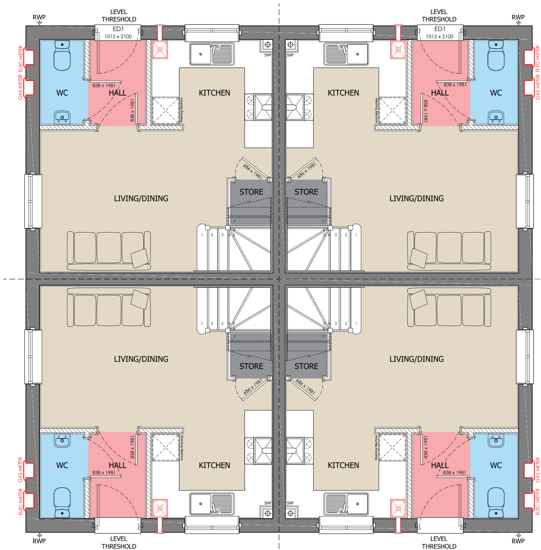
GROUND FLOOR 3 Bed 575Sqt/53.41Sqm
