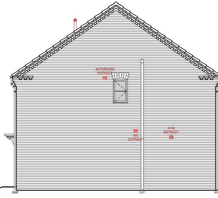
SIDE ELEVATION
