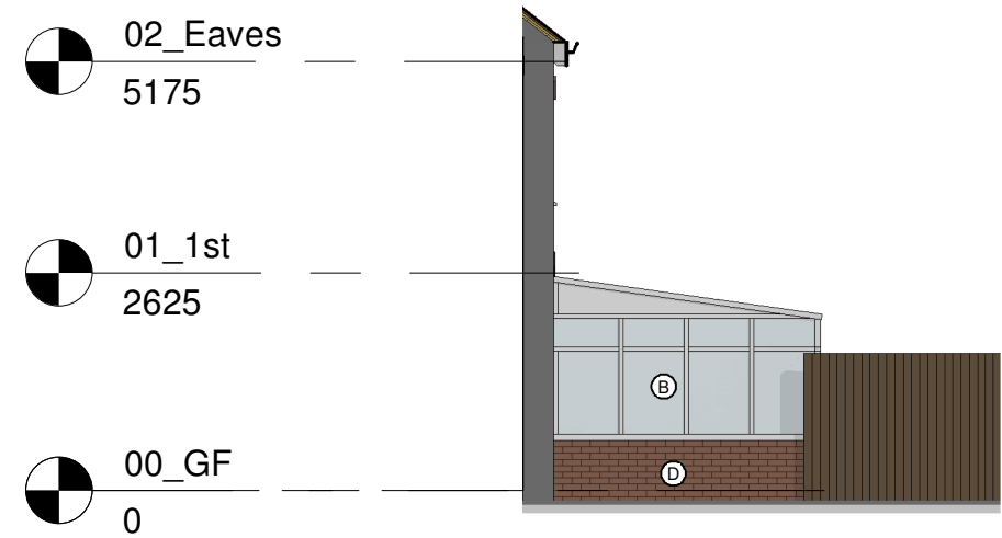
West (Side) Elevation 1 : 100
