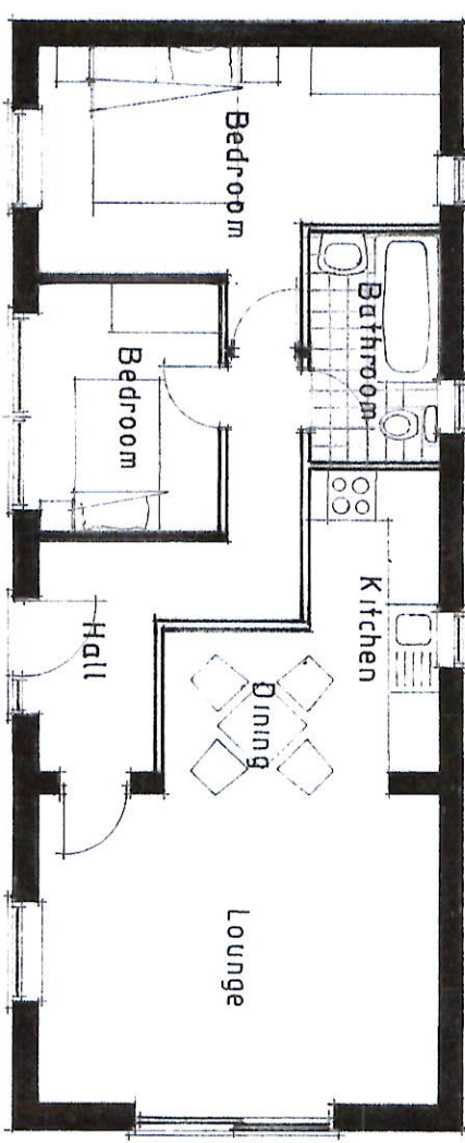
FLOOR PLAN
