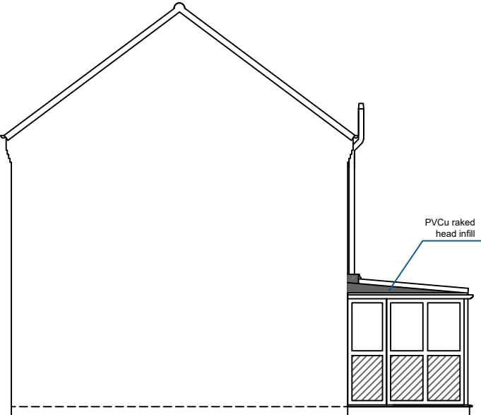
LEFT ELEVATION
