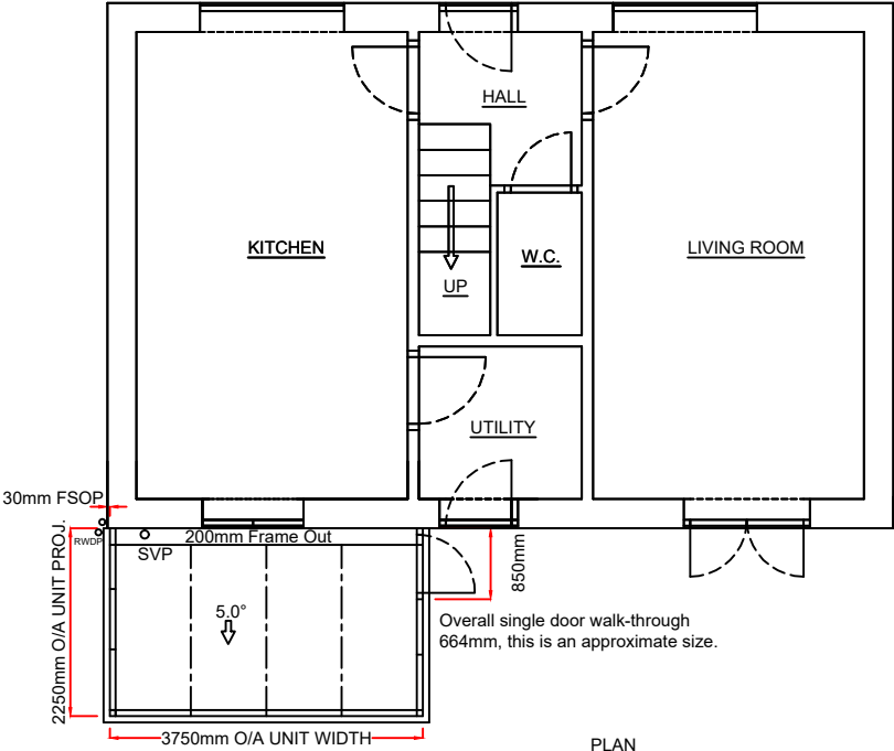
PLAN
