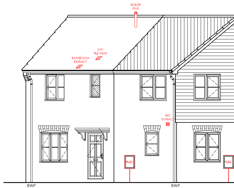
FRONT ELEVATION
