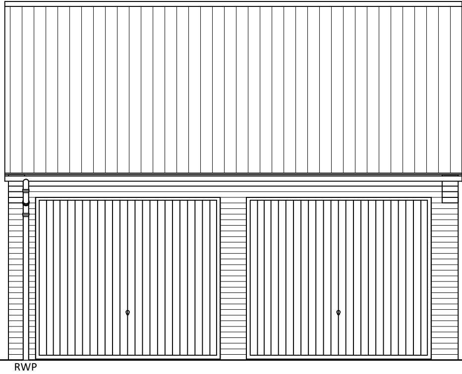
FRONT ELEVATION
