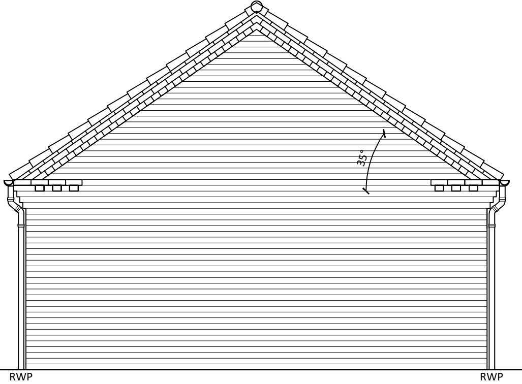
SIDE ELEVATION
