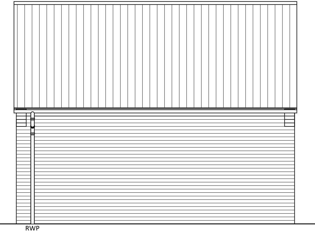
REAR ELEVATION
