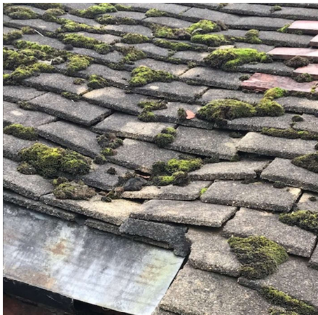
7. Damaged roof structure - to be repaired, remove rotten timbers and replace in matching hardwood.
