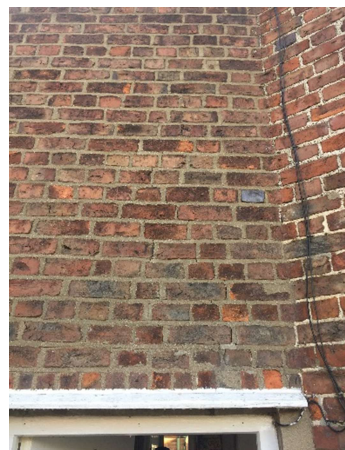
16. Damaged pointing, repoint crack in matching lime mortar.
