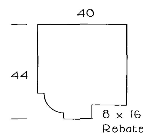
SASH STILE/HEAD
