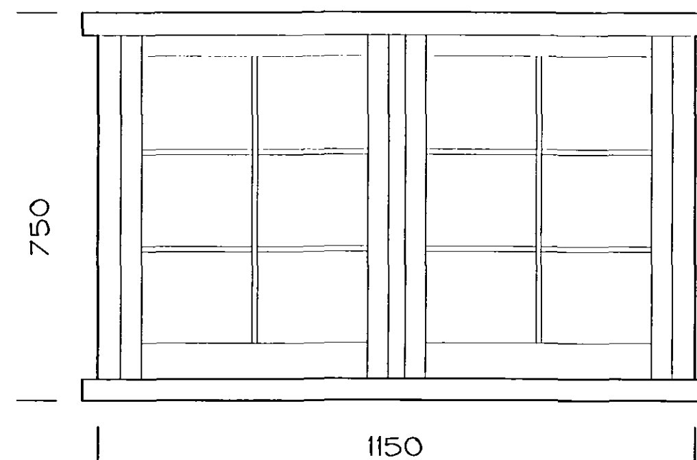
EXISTING ROADSIDE WINDOW ELEVATION DETAIL 1:10
