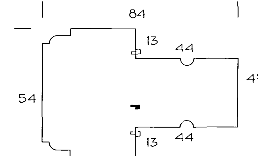
MULLION
