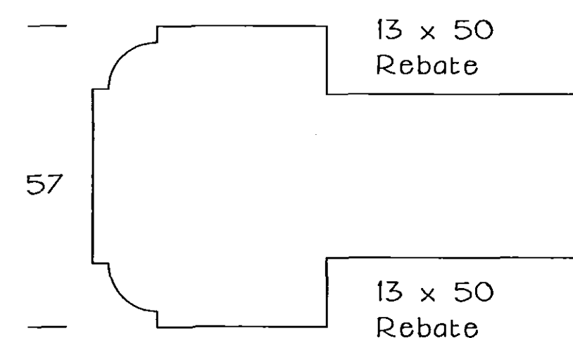
MULLION
