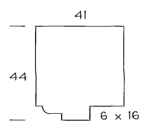
SASH STILE/HEAD
