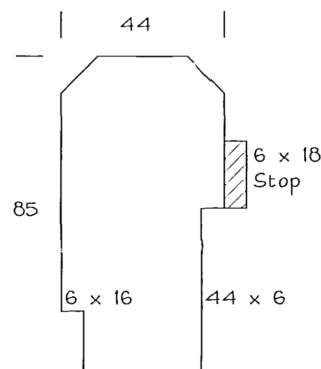
INNER FRAME FOR SASH
