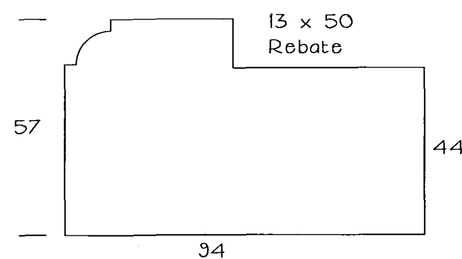
JAMB/HEAD
