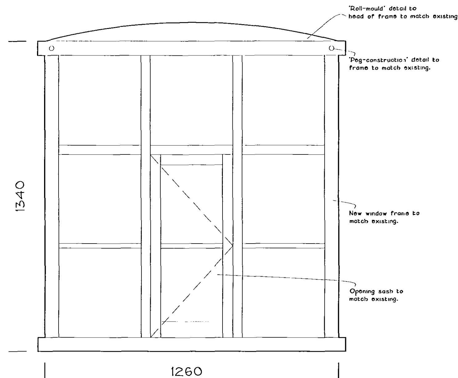
REPLACEMENT LOUNGE WINDOW ELEVATION DETAIL 1:10
