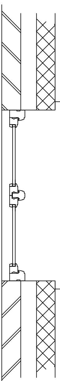
TYPICAL WINDOW CROSS SECTION Condition 7
