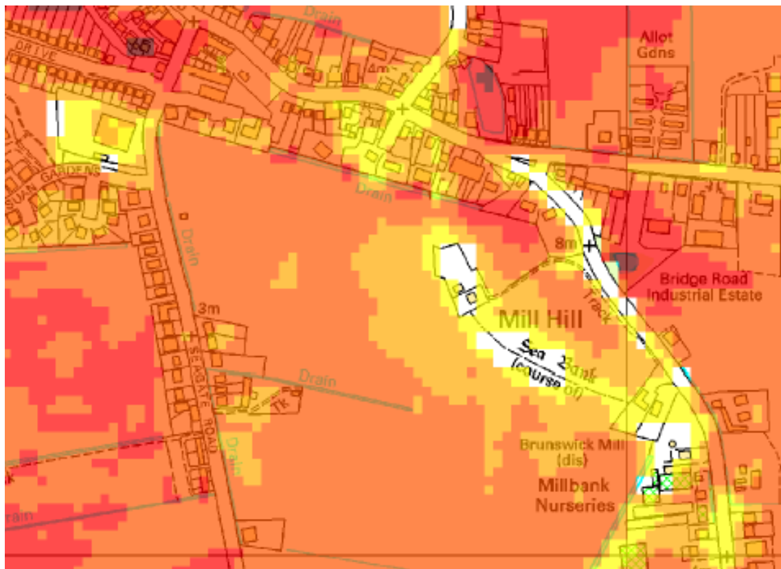
Figure 4- Figure 3- Extract from the 0.1% (1 in 100) Breach Hazard Map showing the majority of the site being within the 0.5-1.0m depth with the central area being in 0.25-0.5m depth
